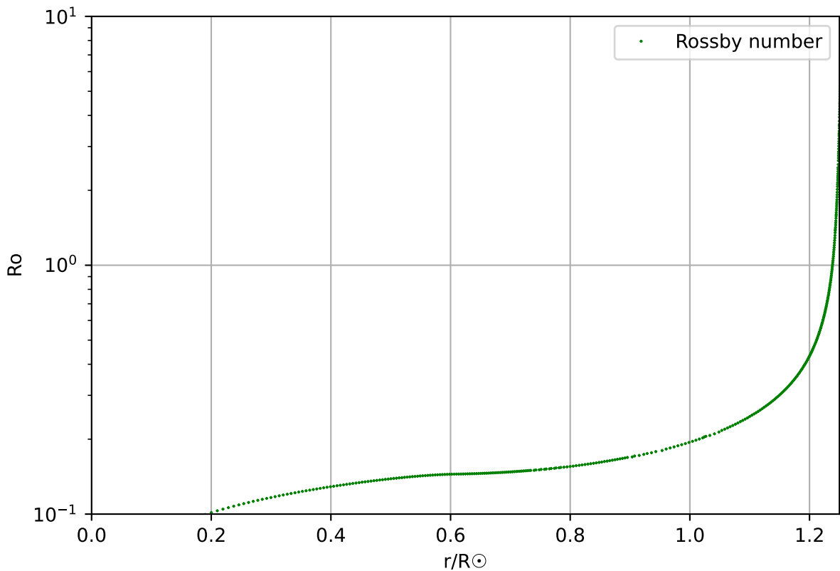
Rossby number, profile 102, age 9.13 \times 10^6
